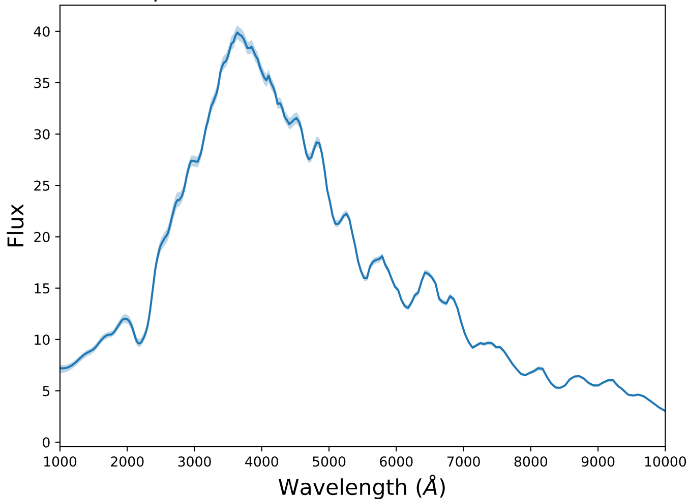
Spectrum 1 for transient CCSN at z=0.41
